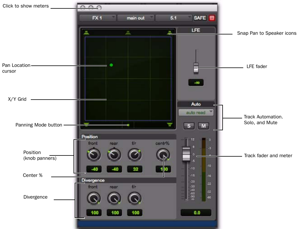
Figure 24. Output window with a 5.1-format multichannel panner
