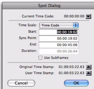
Spot dialog
