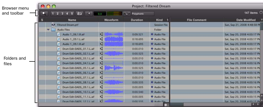
Figure 14. Project browser
