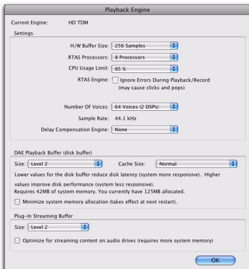
Playback Engine dialog for Pro Tools|HD system
