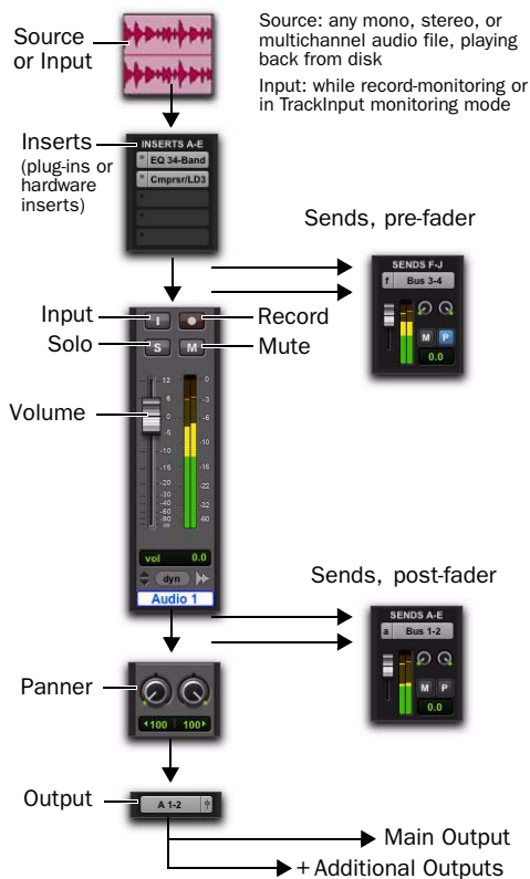
Audio track audio signal flow
