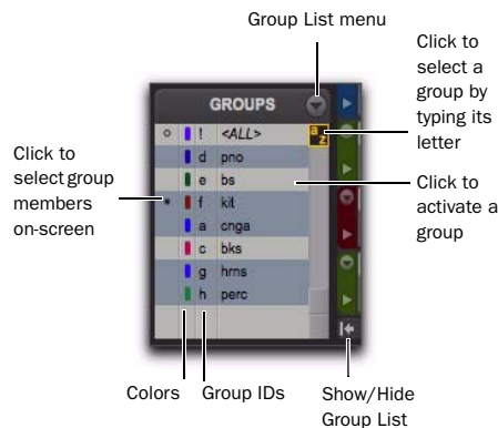
Group List
