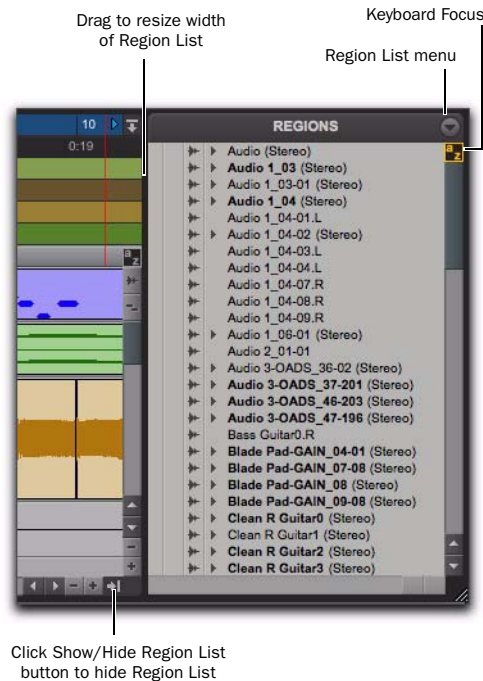
Figure 8. Region List
