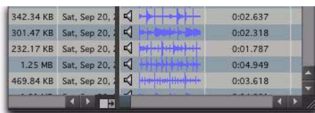
Show/Hide
