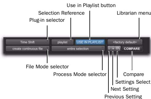
AudioSuite window header
