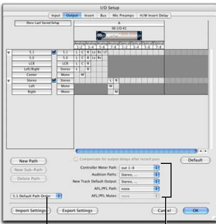
Default selectors in the I/O Setup dialog
