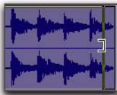
Trimmer tool
