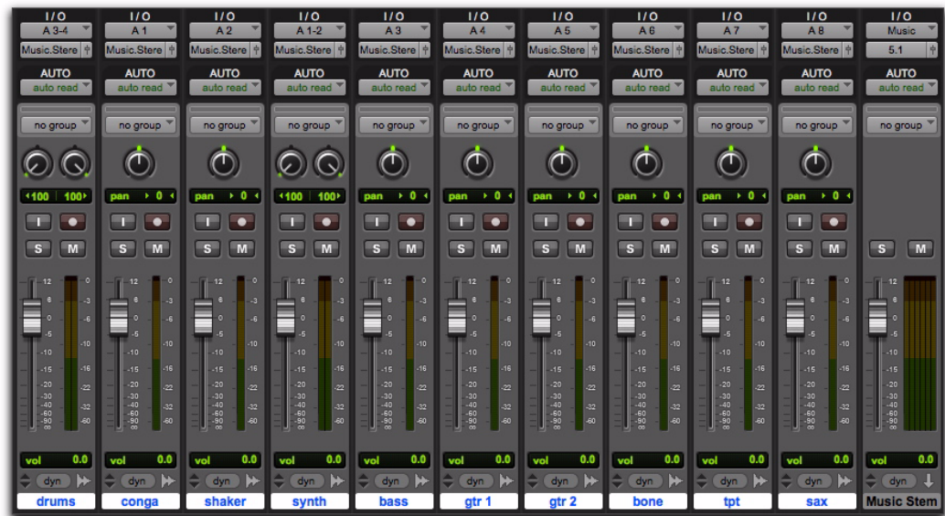
Figure 21. Music stem
